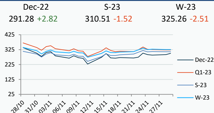
WSI Temperature Forecast c
